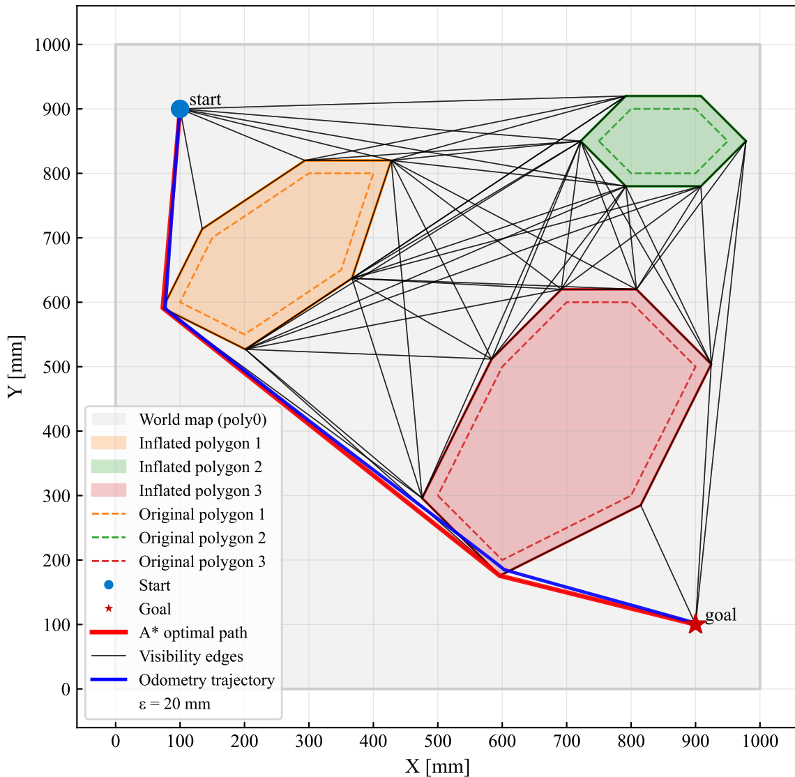
Original vs Inflated Obstacles + Visibility Graph + A* Path + Odometry Trajectory
